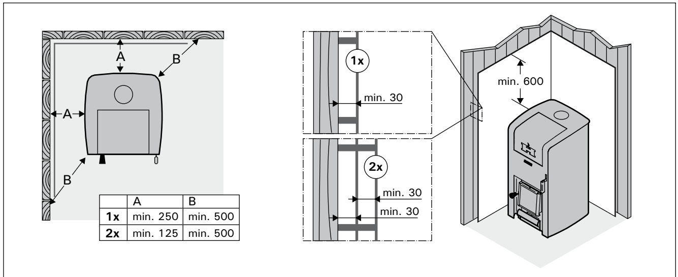
Figure 8. Protective covers (all dimensions in millimeters) Abbildung 8. Schutzabdeckungen (alle Abmessungen in Millimetern)
